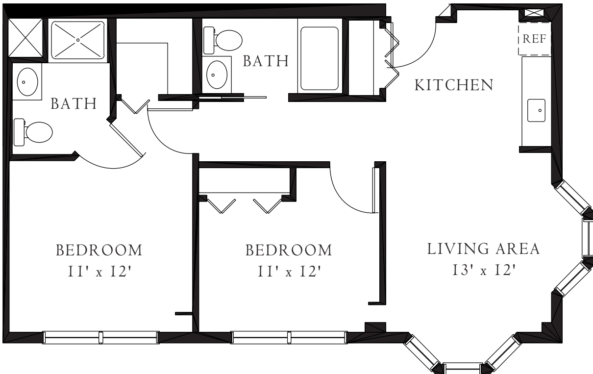
TWO BEDROOM
